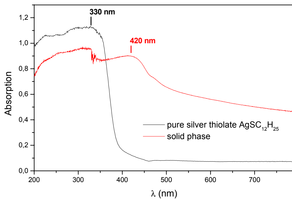
Fig. S2 : UV-visible spectra of pure silver thiolate ( \text{AgSC}_{12}\text{H}_{25} ) and the partially reduced solid phase
