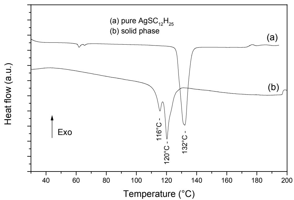
Fig. S3 : Thermal Differential Analysis of the pure silver thiolate and of the partially reduced solid phase.
