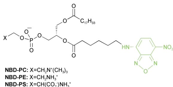
Scheme 9 NBD-labeled phospholipids.
