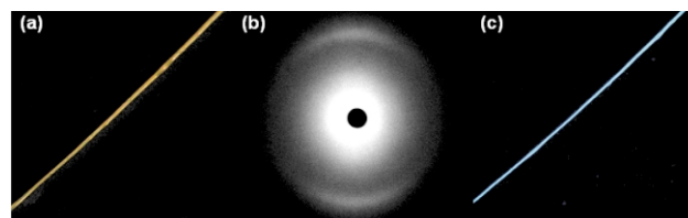
Fig. 3 (a) Optical micrograph (×10) of a fibre obtained from the LC phase of A An -3a-A An and T-3a-T under non-polarized light, (b) fibre diffraction pattern of the fibre and (c) optical micrograph (×100) of the fibre when excited with UV light (365 nm).
