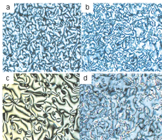
Fig. 2 Polarized optical micrographs of bifringent textures observed for (a) A An 3aA An : T-3a-T at 130 °C; (b) A An 3aA An : T-3b-T at 160 °C; (c) A An -3c-A An : T-3a-T at 155 °C (d) A An -3b-A An : T-3b-T at 120 °C (magnification 500×). See ESI for optical micrographs (×100).†
