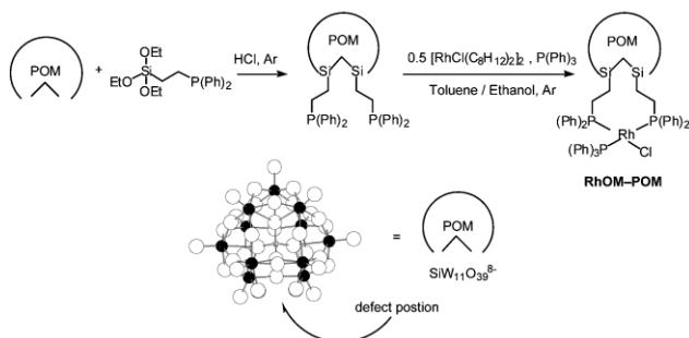
Scheme 1 Synthetic scheme for the preparation of the rhodium based metal-organic-polyoxometalate hybrid compound.
