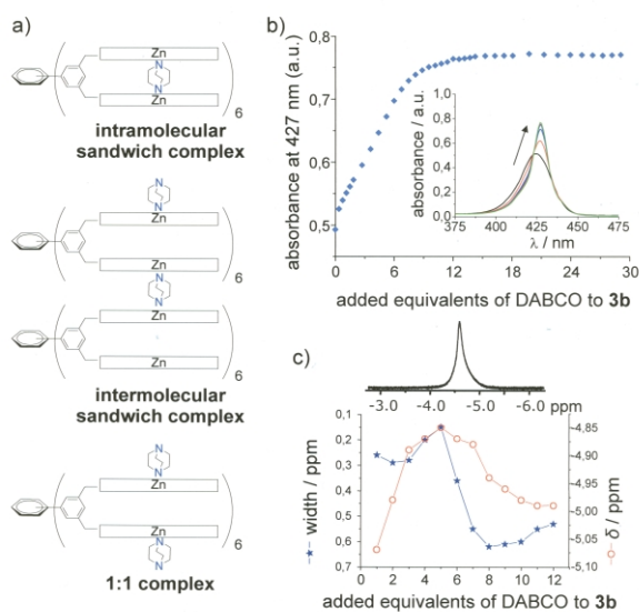
Fig. 2 (a) Schematic representation of possible DABCO : 3b complexes. (b) UV/Vis titration curve of the addition of DABCO to 3b (0.14 \mu M) in chloroform. (c) Top: part of the 1 H-NMR spectrum of 3b with 6 equivalents of DABCO present. Bottom: peak width at half height and chemical shift upon the addition of DABCO to 3b (0.69 mM) in chloroform.
