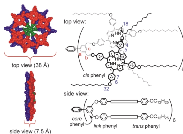
Fig. 1 Left: proposed 'yo-yo'-like shape of 3a in solution (alkyl tails have been omitted for clarity). Right: proton designations and proposed orientation of two porphyrin moieties within 3a as derived from 1D and 2D NMR.
