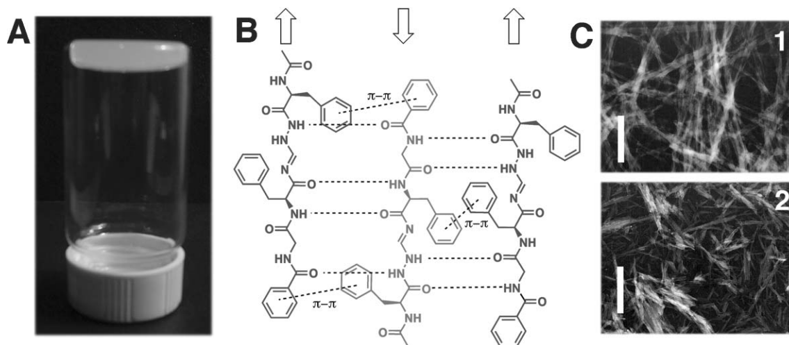
Fig. 2 (A) Organogel formed by 4 mg of 11 in 2 mL of MeOH and 0.2 mL of chlorobenzene. (B) Network of interactions proposed to promote gelation. (C) Negative stain TEM images of organogels formed from 11 (panel 1, 0.3 wt% in 10:1 MeOH:chlorobenzene; panel 2, 0.4 wt% in 1.2:1 DMA:H 2 O); (scale bar 1 μm).
