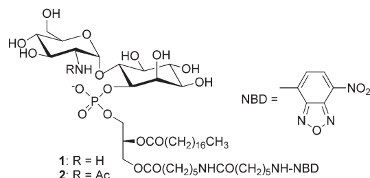
Fig. 2 Structures of NBD-GlcNAc-PI and NBD-GlcN-PI.
