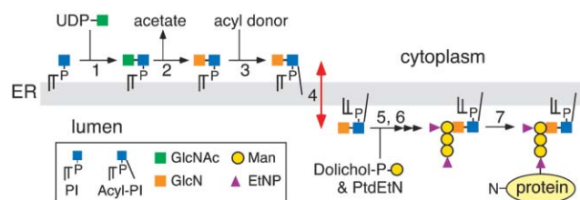
Fig. 1 Topology of GPI biosynthesis in the ER. The first GPI biosynthetic intermediate, GlcNAc-PI, is synthesized (step 1) from PI, then de- N -acetylated (2) to GlcN-PI on the cytoplasmic face of the ER. GlcN-PI or an inositol-acylated derivative (as shown) is proposed to flip across the ER membrane (4). Subsequent elaboration of the structure (5, 6) occurs in the ER lumen where GPI is attached to protein (step 7).
