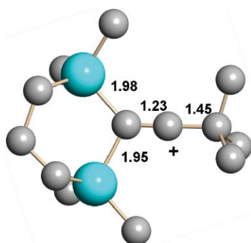
Fig. 7 X-ray structure of a vinyl cation stabilized with t -butyl and \beta -silyl groups. 38
