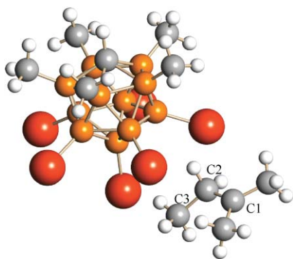
Fig. 6 X-ray structure of the t -pentyl (amyl) cation as a \text{CHB}_{11}\text{Me}_5\text{Br}_6^- carborane salt. \text{C}_1 is the formal \text{sp}^2 cationic centre. 55
