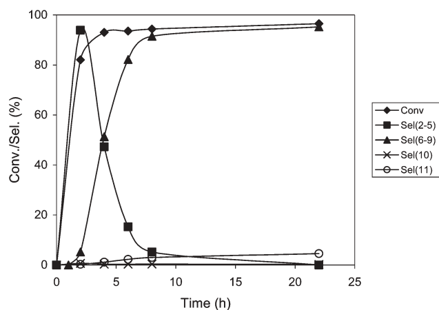
Fig. 3 Hydrogenation of ( \pm )-citronellal over Zr-beta-3%Ni/MCM-41. Reaction conditions as in Fig. 1.
