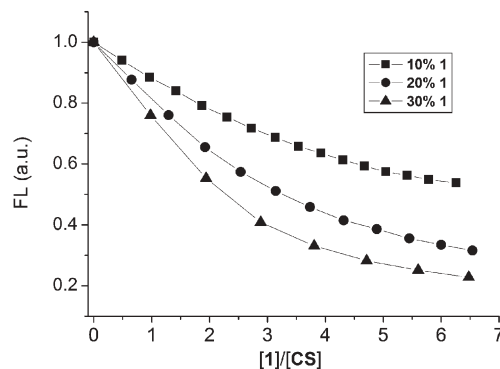
Fig. 1 Fluorescence intensity of CS ligand (10 \mu\text{M} , ex: 400 nm, em: 480 nm) upon titration with POPC vesicles containing different loadings of receptor 1 . ■: 10 mol% 1 ; ●: 20 mol% 1 ; ▲: 30 mol% 1 . All vesicles contained 2 mol% DPPE-PEG-2000 and were in buffer (pH 7.4, 10 mM TES and 145 mM NaCl).
