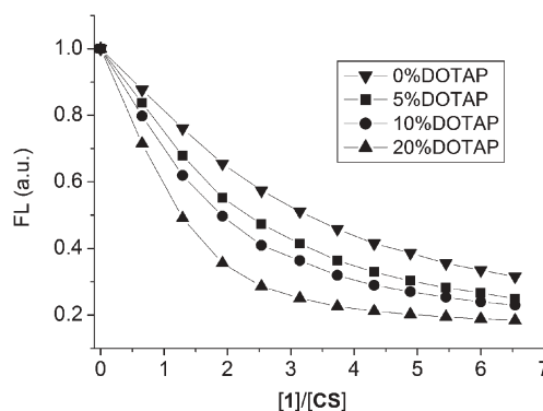
Fig. 3 Fluorescence intensity of CS (10 \mu M, ex: 400 nm, em: 480 nm) upon titration with POPC vesicles containing 20 mol% of 1 and the following amounts of DOTAP: \nabla : 0 mol%; \blacksquare : 5 mol%; \bullet : 10 mol%; \blacktriangle : 20 mol%. All vesicles contained 2 mol% DPPE-PEG-2000 and were in buffer (pH 7.4, 10 mM TES and 145 mM NaCl).
