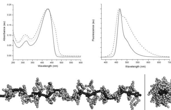
Fig. 2 Top: Normalized absorption and emission spectra of the polymers: PPE-R 1 (solid); PPE-R 1 -COOH (dotted); PPE-R 2 (dashed). Bottom: molecular modelling of PPE-R 1 simulated by Materials Studio 3.0 (Accelrys®). The dark black chain indicates the polymer backbone (left: side view, right: edge view).
