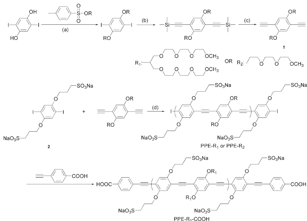
Scheme 1 Polymer synthesis: (a) DMF, K 2 CO 3 , 75 °C, 72 h; (b) THF, Pd(PPh 3 ) 4 , DIPA (diisopropylamine), CuI; (c) KOH, water/methanol.
