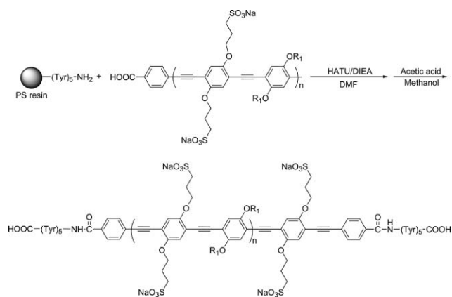
Scheme 2 Peptide-PPE coupling reaction.
