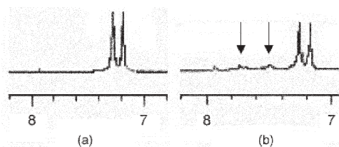
Fig. 1 1 H NMR spectra of PPE-R 1 in D 2 O (a) before and (b) after end-capping.
