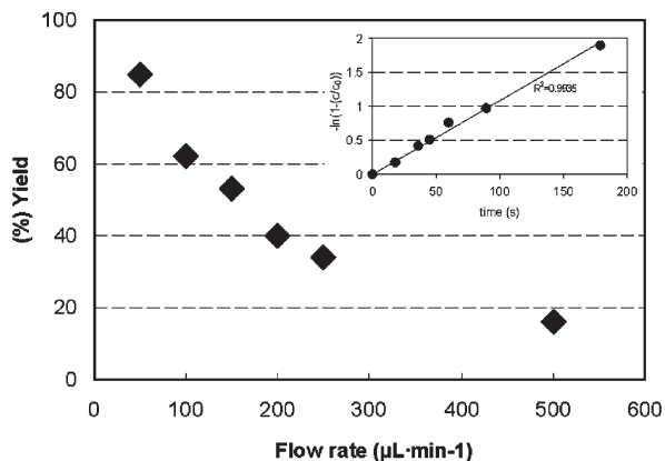
Fig. 3 % Yield 7a vs. flow rate for the continuous Heck reaction between 5 and 6a in ethanol at 200 °C and 8 MPa, 0.67 mol L -1 of 5 . Kinetics data showing a pseudo first order rate K_{\text{obs}} = 10.8 \times 10^{-3} \text{ s}^{-1} (38.9 h -1 ).
