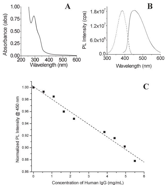
Fig. 2 (A) Absorption spectrum of AuQDs, 1 cm cell pathlength; (B) Excitation and emission spectra of AuQDs in aqueous solution, 1 cm cell pathlength, pH = 6.3: excitation (---) and emission (—) (C) Quenching of AuQDs conjugated with goat-derived polyclonal anti-human IgG PL with increasing concentration of human IgG.
