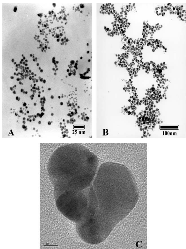
Fig. 3 (A) HRTEM micrograph of AuQD-antibody conjugates, data bar size 25 nm (B) HRTEM micrograph of the complex agglomerate formed after addition of recombinant human IgG protein to the AuQD-antibody conjugate, data bar size 100 nm. (C) HRTEM micrograph of AuQD-antibody conjugates showing density differences due to PAMAM and Au, data bar size 5 nm.
