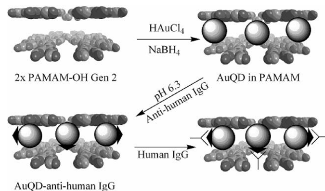
Fig. 1 Schematic representation of PAMAM-OH dendrimer, generation 2, AuQD formation between dendrimers, Conjugation of anti-human IgG (▲) to the AuQD-PAMAM complex, and addition of human IgG (Y) to the system.
