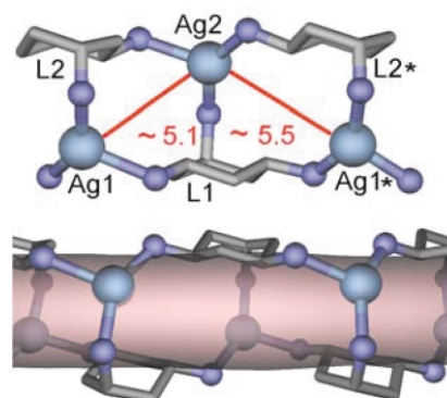
Fig. 1 Top: macrocycle formation of 1 . Bottom: 1-D coordination polymer of 1 . Ag atoms are shown as large blue circles, carbon in grey and nitrogen as small blue circles. Symmetry code *: x, 1+y, z . Each Ag(I) adopts a trigonal planar coordination sphere (N–Ag1–N angles: 147.92(17), 114.35(17), 97.47(17)° \Sigma = 359.74(17)^\circ and N–Ag2–N: 148.32(16), 108.14(16), 103.08(16)° \Sigma = 359.54(16)^\circ ) by coordinating two equatorial and one axial amino group of three different ligands.
