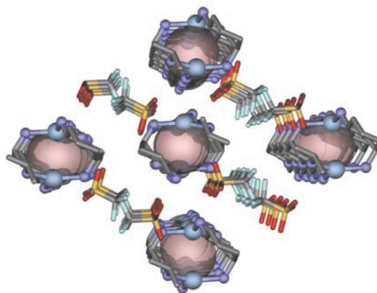
Fig. 2 Packing arrays of 1 along the crystallographic b axis. Ag(I) atoms are shown as large blue circles, carbon in grey, sulfur in yellow, oxygen in red, fluoride in light blue and nitrogen as small blue circles.
