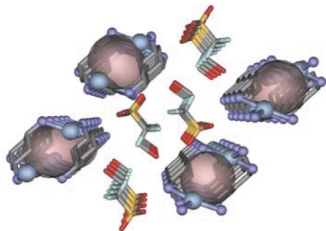
Fig. 4 Packing arrays of 2 along the crystallographic b axis. Ag(I) atoms are shown as large blue circles, carbon in grey, sulfur in yellow, oxygen in red, fluoride in light blue and nitrogen as small blue circles.
