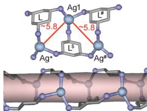
Fig. 3 Top: macrocycle formation of 2 . Bottom: one-dimensional coordination polymer of 2 . Ag atoms are shown as large blue circles, carbon in grey and nitrogen as small blue circles. Symmetry codes *: 3/2-x , -1/2+y , 3/2-z , #: 3/2-x , 1/2+y , 3/2-z and $: x , -1+y , z . Each Ag(I) ion has a trigonal planar coordination sphere (N–Ag–N angles: 102.42(10), 106.94(10), 150.33(11)° \Sigma = 359.69(11)°) with three cis -amines of different ligands forming the channel (Ag–N1, N2, N3 distances: 2.232(3), 2.230(3), 2.393(3) Å, respectively).
