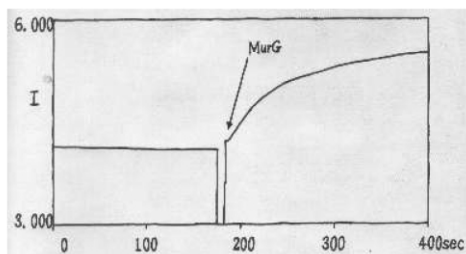
Fig. 2 Progress of MurG catalysed reaction upon addition of 3.0 \mu\text{g} MurG to 3.0 \mu\text{M} dansyl lipid 1 and 2.7 \mu\text{M} 1 .
