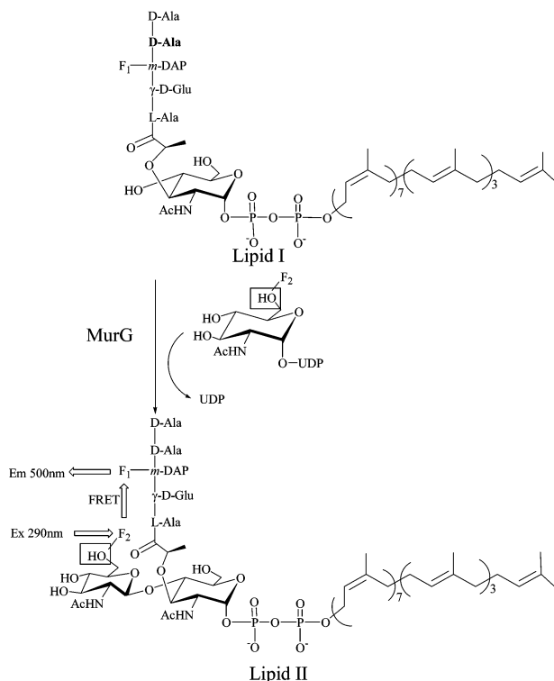
Fig. 1 MurG catalysed reaction. In the FRET assay, the dansyl fluorophore (F 1 ) acceptor is attached to position 3 of pentapeptide, the indole-3-acetic acid fluorophore (F 2 ) donor is attached to the C-6 position of UDP-GlcNAc.
