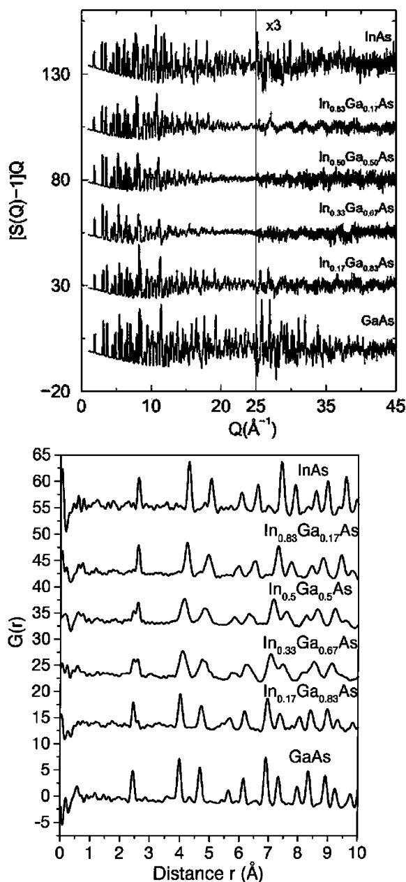
Fig. 3 (a) The reduced total scattering structure functions [S(Q)-1]Q for \text{In}_x\text{Ga}_{1-x}\text{As} measured at 10K. The data-sets from the different members of the alloy series are offset for clarity. The high- Q region is shown on an expanded scale ( \times 3 ) to highlight the presence of the diffuse scattering. (b) The PDFs, G(r) , obtained from the data in (a) by Fourier transformation. Note the nearest neighbor peak is split into two components in the alloys.
