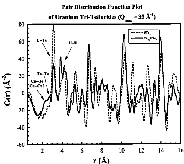
Fig. 15 PDF data obtained for \alpha - \text{UTe}_3 and \text{Cu}_{0.33}\text{UTe}_3 .
