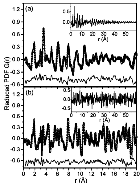
Fig. 11 Experimental (circles) and fitted (solid line) PDFs for (a) V 2 O 5 ·nH 2 O xerogel and (b) crystalline V 2 O 5 . The residual difference is shown in the lower part. The experimental data are shown over longer range in the insets to emphasize the nanocrystalline nature of the xerogel (inset in (a)).
