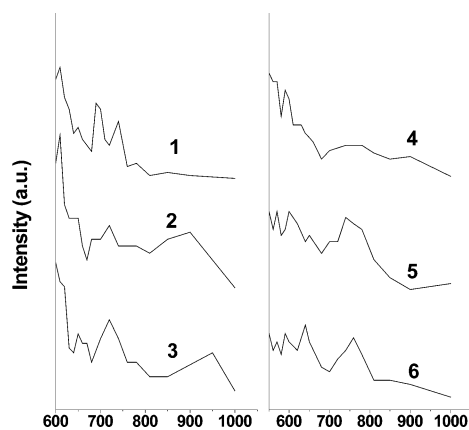
Fig. 2 Two-photon absorption.
