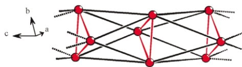
Fig. 3 The magnetic framework of 1 and 2 with halide-mediated intra-triangle exchanges (red bonds) and halide-amino-mediated inter-triangle exchanges (black bonds, intra/inter-triangle \text{Cu}\cdots\text{Cu} distances: 4.46/6.82 Å).
