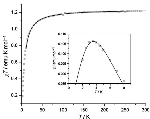
Fig. 4 Temperature dependence of \chi T at 0.1 Tesla for compound 2 . The solid line, superimposed over the experimentally derived values (grey squares), represents the fit of the high-temperature data (10–290 K) to the Heisenberg model for an equilateral \{\text{Cu}^{\text{II}}_3\} triangle. The inset shows the observed low- T maximum around 3.5 K in the temperature dependence of the molar susceptibility with a best fit to the Bonner–Fisher model of an equidistant linear S = \frac{1}{2} Heisenberg chain for the 2–7 K interval.
