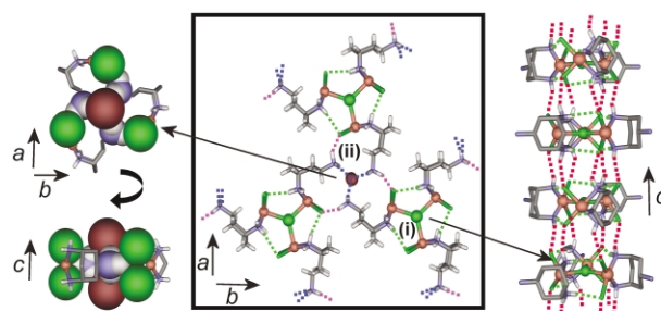
Fig. 2 The central view shows the 2-D network with the hydrogen bonded halide counter-ions in the centre linking three \{\text{Cu}^{\text{II}}_3\text{Cl}\} triangular cluster units (i) via the different classes of hydrogen bonded interactions (coloured dotted lines). The left views show the primary coordination sphere around the hydrogen bonded halides (ii) (halides and nitrogen atoms shown as CPK); the top view is shown projected onto the ab plane and the bottom view is perpendicular to the c axis. The right view shows a representation of the 1-D chains formed between the \{\text{Cu}^{\text{II}}_3\text{Cl}\} cluster units that run parallel to the c axis. H: white, Cl: green, N: blue, C: grey, Cu: pink, Cl/Br sites in 1 and 2 , respectively: brown.
