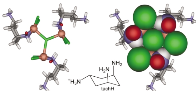
Fig. 1 Representations of the triangular clusters present in 1 and 2 (left: stick representation, the Cu ions are shown as spheres; right: CPK overlay of the primary coordination sphere). The non-coordinated hydrogen bonded halide counter-ions are omitted. (Cl: green, N: blue, C: grey, Cu: pink). The H positions are shown in white except those that are involved in the formation of the Heisenberg chains, shown in red.
