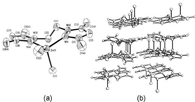
Fig. 1 (a) ORTEP representation of [Zn(bmpze)Cl 2 ] (50% probability ellipsoids) with atom numbering scheme. (b) Packing diagram showing two kinds of planes parallel to bc .
