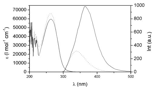
Fig. 2 Absorption and emission spectra for compound L 2e (dotted line) and [Zn(L 2e )Cl 2 ] (solid line).
