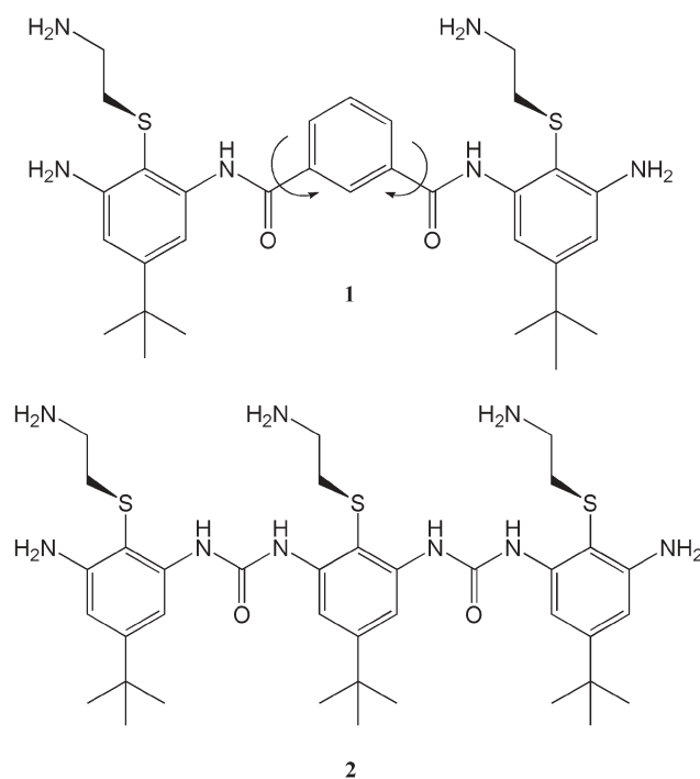
Fig. 1 The structure of arylamide 1 and urea trimer 2 .
