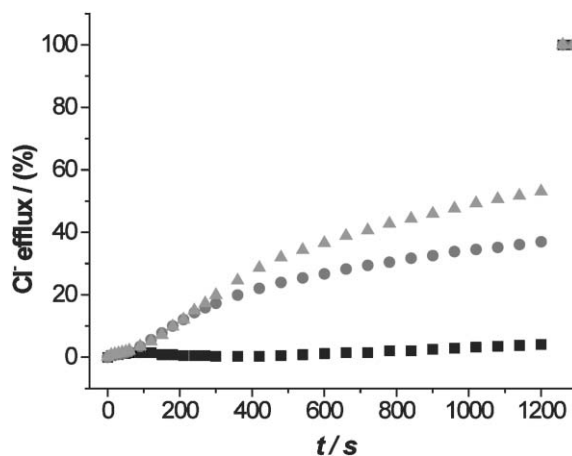
Fig. 3 \text{Cl}^- efflux induced by the addition of 2 ( 10 \mu\text{M} ) to vesicles containing NaCl (500 mM), \text{X}_1 solution, and dispersed in \text{NaNO}_3 (500 mM), \text{X}_2 solution. ■ \text{X}_1 and \text{X}_2 = citric acid (5 mM), pH 4.0; ● \text{X}_1 and \text{X}_2 = citric acid (5 mM), pH 7.2; ▲ \text{X}_1 = citric acid (5 mM), pH 4.0, \text{X}_2 = sodium phosphate (5 mM), pH 6.7. At t = 1300 s, the vesicles were lysed to produce 100% \text{Cl}^- release.
