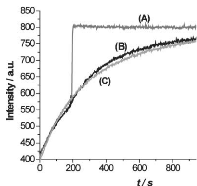
Fig. 4 Change in Oregon Green ® 514 fluorescence upon addition of: (A) 2 (10 \mu\text{M} ), (B) 3 (8.8 \mu\text{M} ), and (C) no receptor, at t = 200 s to vesicles containing Oregon Green (10 \mu\text{M} ), NaCl (500 mM), and citric acid (5 mM), pH 4.0. The vesicles were dispersed in an external solution of \text{NaNO}_3 (500 mM), and sodium phosphate (5 mM), pH 7.2.
