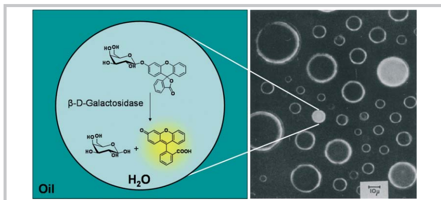
Fig. 1 The first measured activity of a single enzyme. A highly diluted, aqueous enzyme solution containing a pro-fluorescent substrate is sprayed into silicone oil. After incubation, some droplets show fluorescence whereas others remain dark. The fluorescence intensity shows discrete levels, depending on the number of active enzymes present in each droplet. By choosing the enzyme concentration such that most droplets contain either zero or one enzyme molecule, the activity of a single enzyme molecule can be determined.
