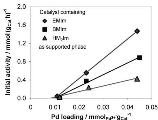
Fig. 2 Catalytic activity of the Lewis/Brønsted bi-functional catalysts in the addition of aniline to styrene (slurry phase, 125 °C).
