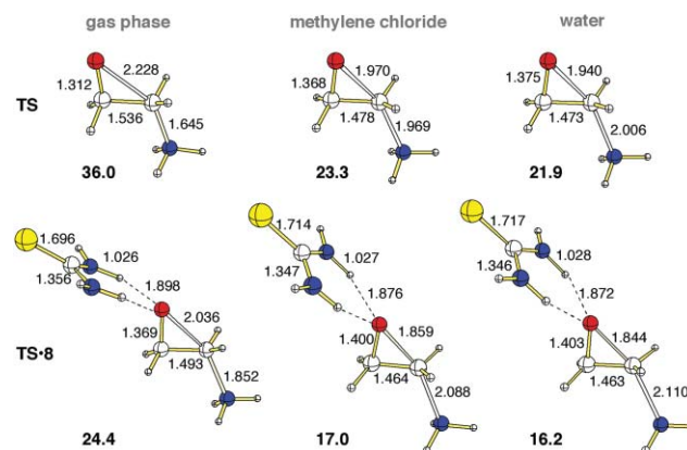
Fig. 3 TSs for uncatalyzed and thiourea-catalyzed epoxide openings in the gas phase, CH 2 Cl 2 , and water at B3LYP/6-311++G(d,p)//B3LYP/6-31G(d) (SCRF solvent inclusion). Selected bond distances in Å. Activation barriers (bold) in kcal mol -1 . Red = O, white = C/H, blue = N, yellow = S.
