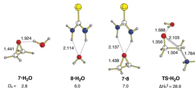
Fig. 2 Hydrogen bonded complexes of the reactants with dissociation energies ( D 0 ) and the TS for the water-catalyzed opening of 7 at B3LYP/6-311++G(d,p)//B3LYP/6-31G(d).
