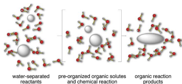
Fig. 1 Hydrophobic hydration: minimization of water ordering.
