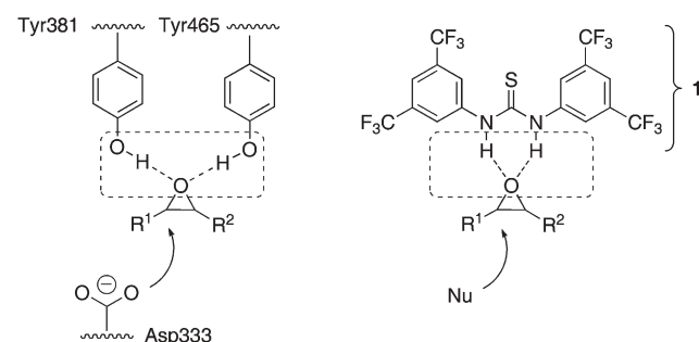
Scheme 1 Epoxide recognition for epoxide hydrolase and 1 .
