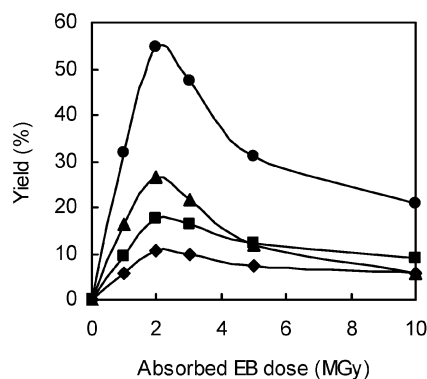
Fig. 2 Yields of each amine converted from benzenesulfonamide (BSA) within the \beta -CD inclusion complex plotted as a function of the absorbed EB dose: o - and p -Fries products ( \blacklozenge and \blacksquare , respectively), aniline ( \blacktriangle ), and the total of them ( \bullet ).
