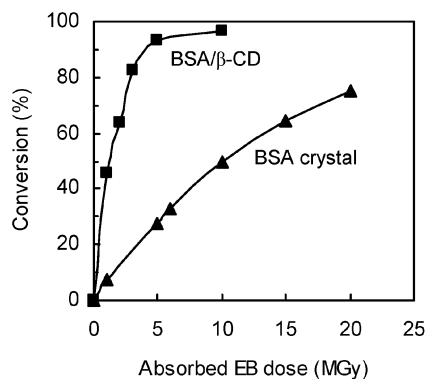
Fig. 1 Conversions of benzenesulfonamide (BSA) in the crystalline state and the \beta -CD inclusion complex (BSA/ \beta -CD) under EB irradiation (1 MeV, 1 mA).
