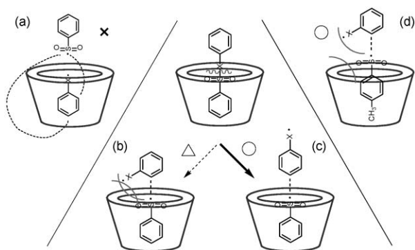
Fig. 3 Proposed mechanism of the EB-Fries rearrangement of sulfonamide and sulfonate within \beta -CD inclusion complexes: (a)–(c) BSA/ \beta -CD, (d) TSA/ \beta -CD and PTS/ \beta -CD.
