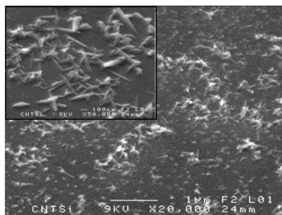
Fig. 2 SEM images of MWNTs bound to Si(111) surfaces.
