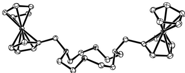
Fig. 1 ORTEP 17 view of 4 showing thermal ellipsoids at a 50% probability level. Hydrogen atoms are omitted for clarity.
