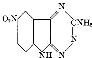
3-Amino-6-Nitroindotriazine
