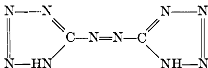
Azotetrazole
