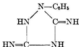
1-Phenyl-3,5-diaminodihydrotriazole
