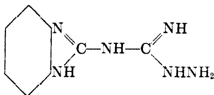
o -Phenyleneaminobiguanide
