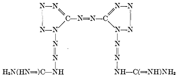
Bis-1,1(3-guanyltriazeno)-5,5-azotetrazole
