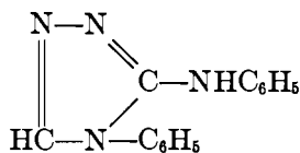
4-Phenyl-5-aniltriazole
