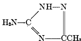
Aminomethyltriazole
