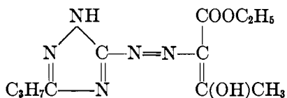
Ethyl 3-propyl-1,2,4-triazole-5-azoacetoacetate
