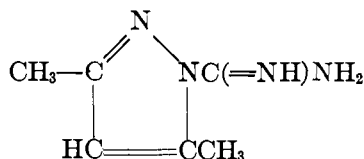
3,5-Dimethyl-2-guanylpyrazole
