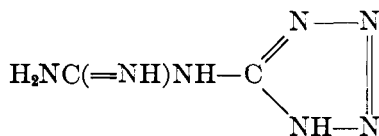
Guanylaminotetrazole
