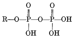
Organic pyrophosphate
