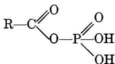
Carboxyl phosphate
