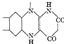
Dihydroalloxazine
