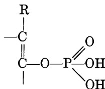
Enolic phosphate
