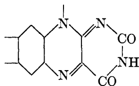
Alloxazine
