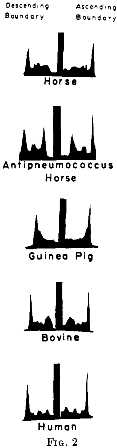
FIG. 2. Electrophoretic schlieren patterns of human, bovine, guinea pig, and horse sera
