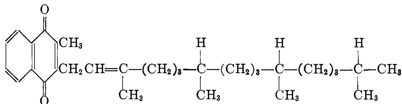
IV Vitamin K 1 or 2-methyl-3-phytyl-1,4-naphthoquinone
