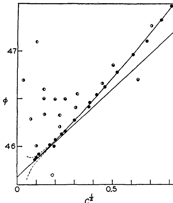
Fig. 1. Apparent molal volumes of potassium chlorate. \circ , International Critical Tables Vol. III (25°C.); \ominus , Joy and Wolfenden (19) (interpolated to 25°C.); \bullet , Jones and Talley (17) (25°C.); \odot , Jones and Ray (18) (25°C.); \bullet , this paper (24.81°C.).
