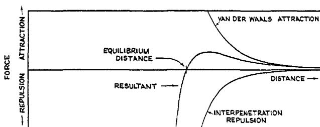
FIG. 1. Illustrating the variation with the distance between two atoms of their mutual van der Waals attraction and interpenetration repulsion forces and of the resultant force.
