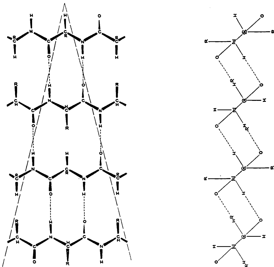
FIG. 4. Two views of another hypothetical pattern for a layer of extended polypeptide chains.
