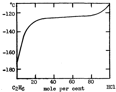
FIG. 26. Ethane-hydrogen chloride system
