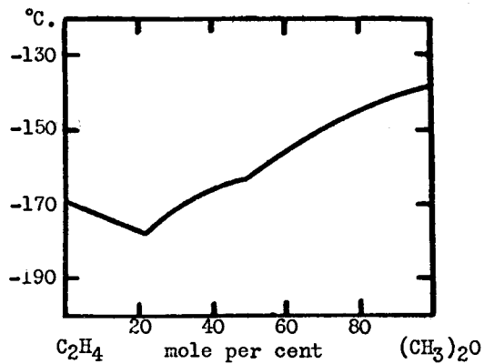
FIG. 29. Ethylene-methyl ether system
