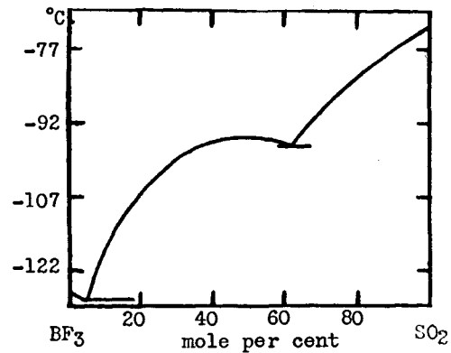
FIG. 18. Boron trifluoride-sulfur dioxide system
