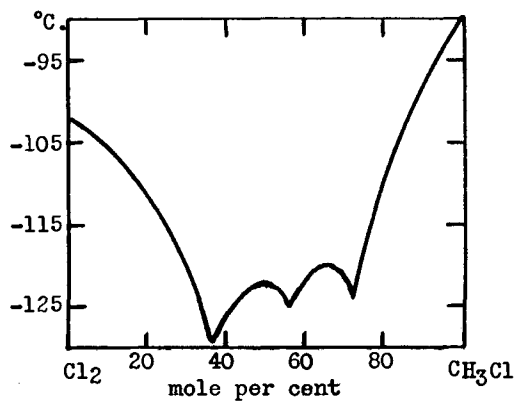
FIG. 23. Chlorine-methyl chloride system
