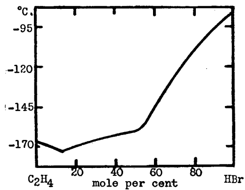
FIG. 27. Ethylene-hydrogen bromide system
