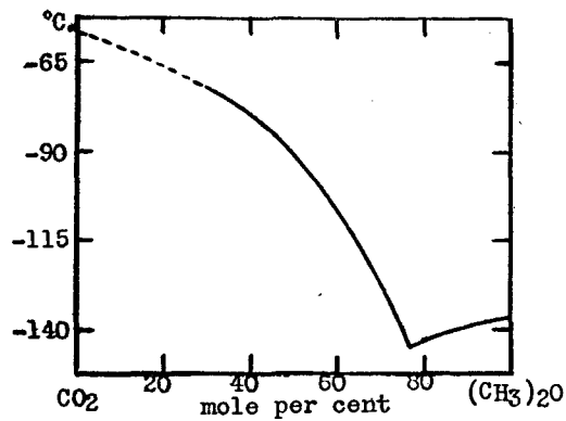
FIG. 20. Carbon dioxide-methyl ether system
