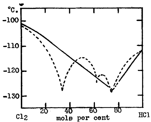
FIG. 22. Chlorine-hydrogen chloride system
