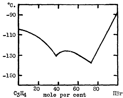
FIG. 5. Allylene-hydrogen bromide system
