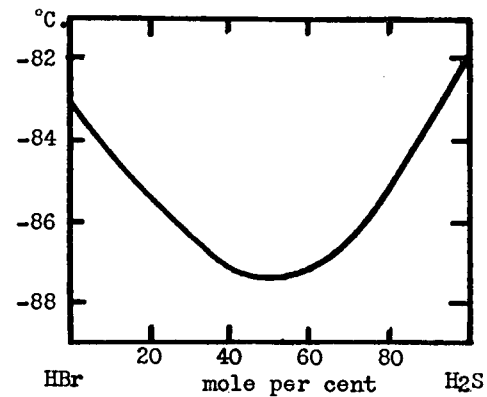
FIG. 30. Hydrogen bromide-hydrogen sulfide system
