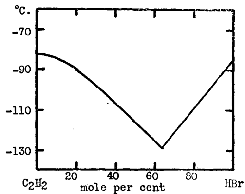
FIG. 3. Acetylene-hydrogen bromide system
