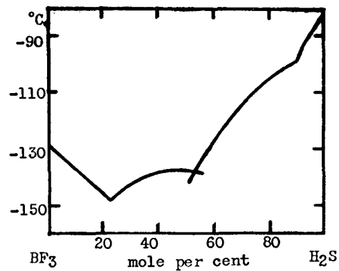
FIG. 14. Boron trifluoride-hydrogen sulfide system
