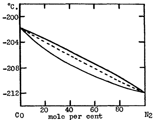
FIG. 21. Carbon monoxide-nitrogen system
