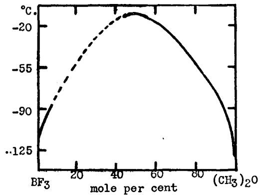
FIG. 16. Boron trifluoride-methyl ether system
