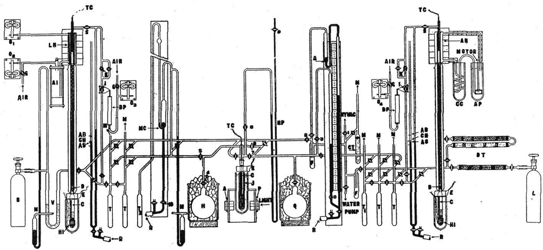
FIG. 1. Typical apparatus used for thermal analysis of liquefied gases
