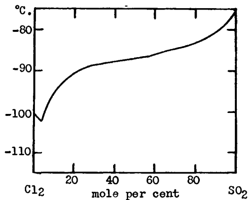
FIG. 25. Chlorine-sulfur dioxide system
