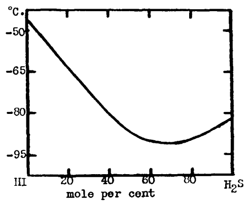
FIG. 37. Hydrogen iodide-hydrogen sulfide system
