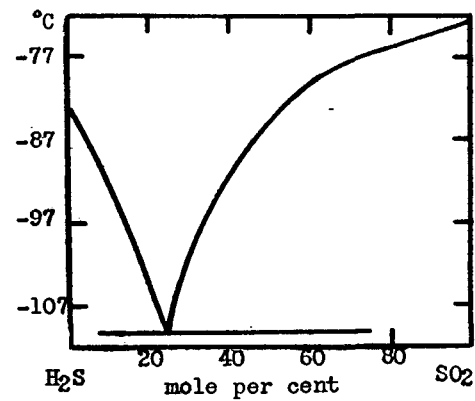
FIG. 40. Hydrogen sulfide-sulfur dioxide system
