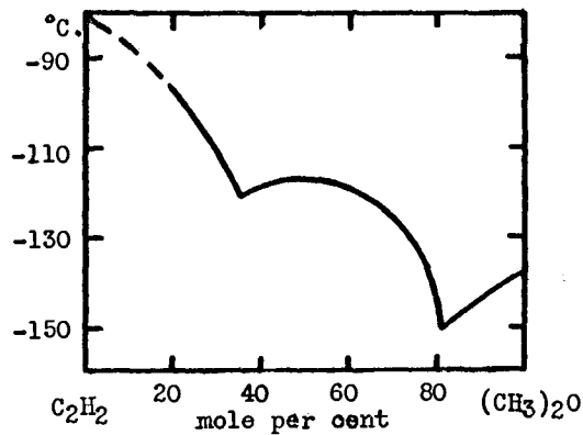
FIG. 4. Acetylene-methyl ether system
