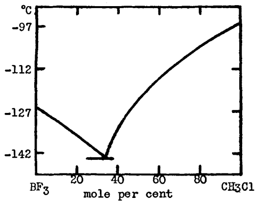
FIG. 15. Boron trifluoride-methyl chloride system
