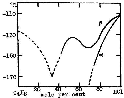
FIG. 19. Butylene-hydrogen chloride system
