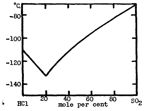
FIG. 36. Hydrogen chloride-sulfur dioxide system
