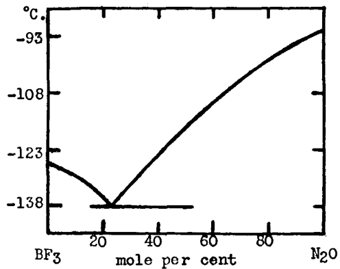
FIG. 17. Boron trifluoride-nitrous oxide system
