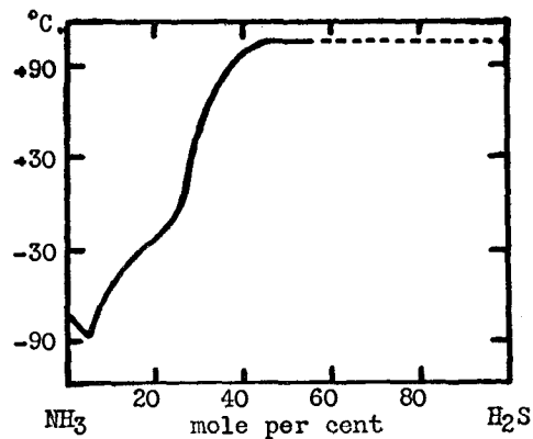
FIG. 6. Ammonia-hydrogen sulfide system
