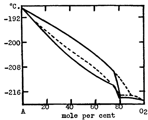
FIG. 12. Argon-oxygen system
