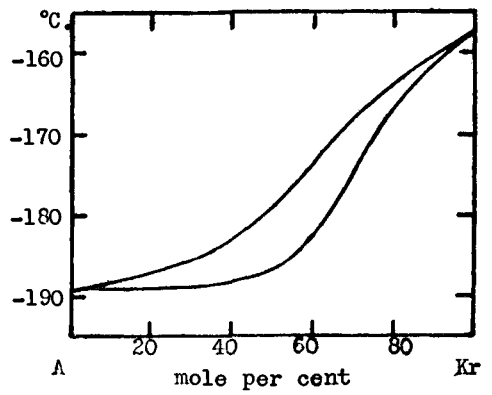
FIG. 9. Argon-krypton system
