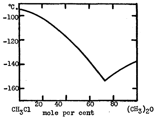
FIG. 43. Methyl chloride-methyl ether system
