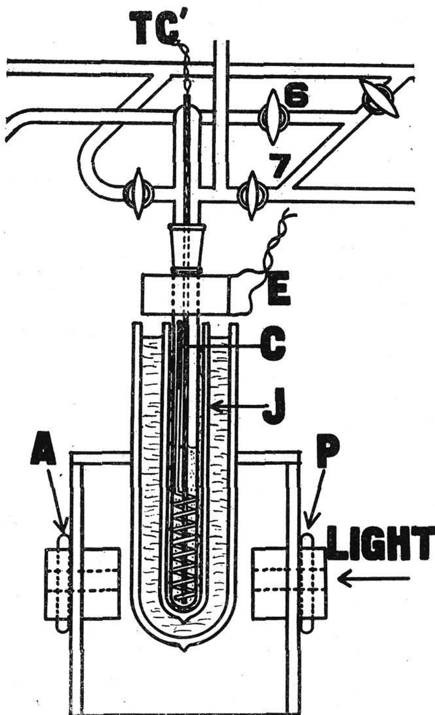
FIG. 2. The freezing-point cell
