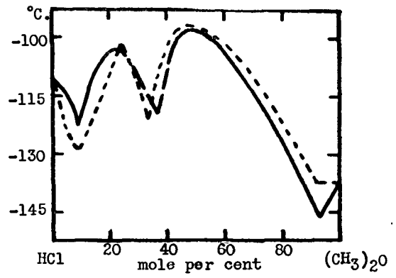
FIG. 35. Hydrogen chloride-methyl ether system
