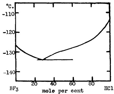
FIG. 13. Boron trifluoride-hydrogen chloride system
