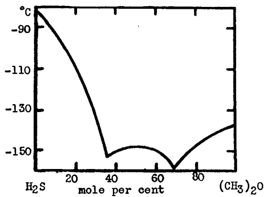
FIG. 39. Hydrogen sulfide-methyl ether system
