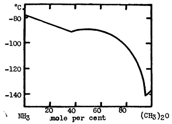
FIG. 7. Ammonia-methyl ether system
