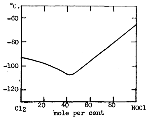
FIG. 24. Chlorine-nitrosyl chloride system
