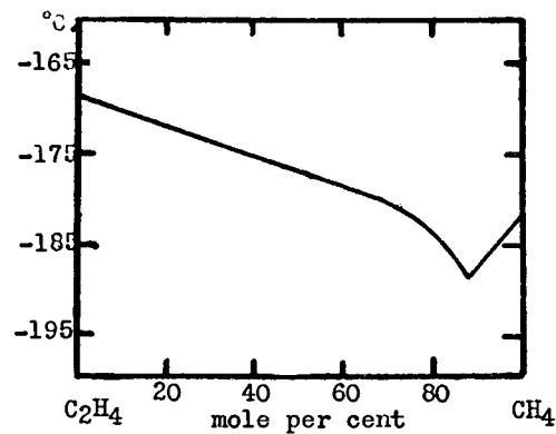
FIG. 28. Ethylene-methane system
