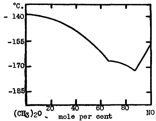
FIG. 44. Methyl ether-nitric oxide system
