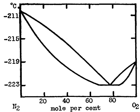
FIG. 46. Nitrogen-oxygen system
