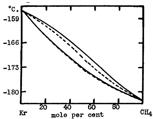
FIG. 41. Krypton-methane system
