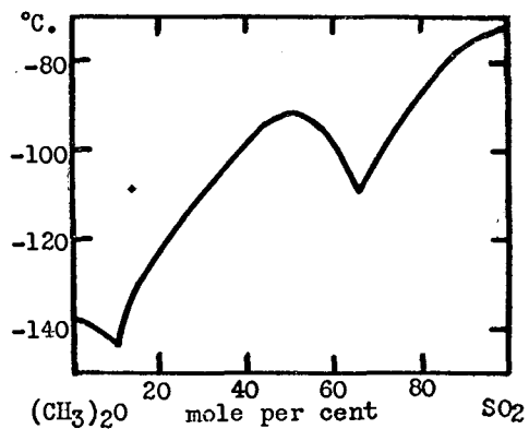
FIG. 45. Methyl ether-sulfur dioxide system
