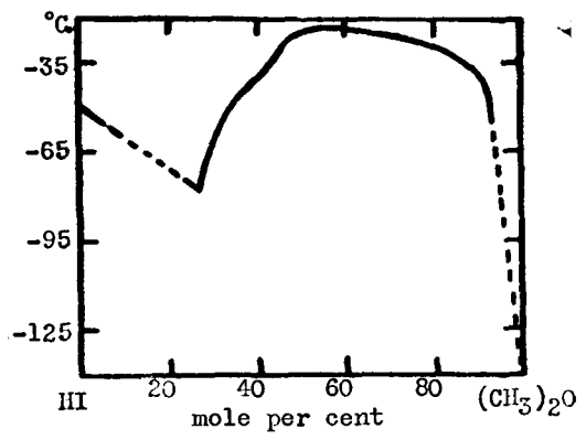
FIG. 38. Hydrogen iodide-methyl ether system
