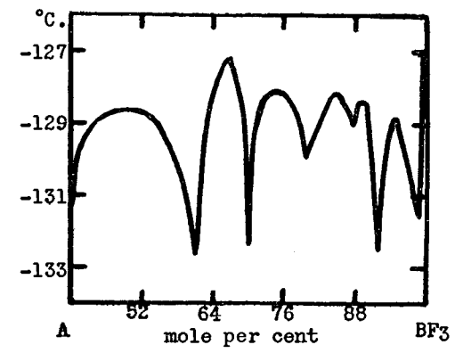
FIG. 8. Argon-boron trifluoride system
