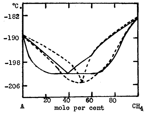
FIG. 10. Argon-methane system
