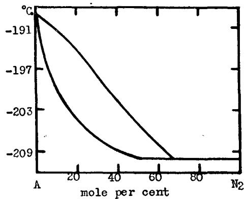
FIG. 11. Argon-nitrogen system
