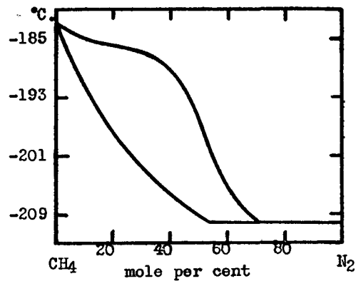
FIG. 42. Methane-nitrogen system
