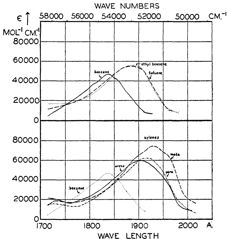
FIG. 1. Transitions near 1900 A. in alkylbenzenes
