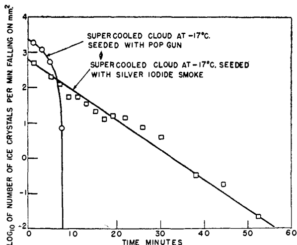
FIG. 4. Comparison of seeding with silver iodide smoke and seeding with popgun
