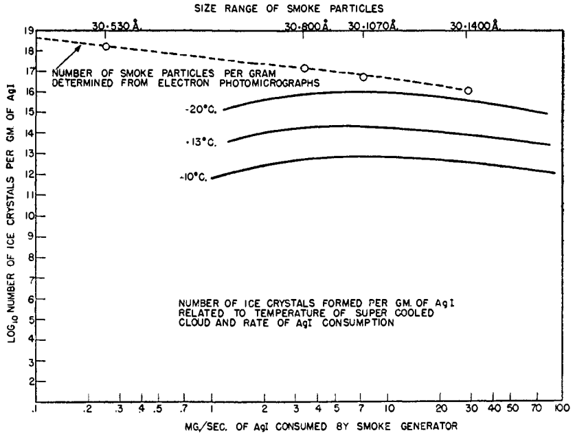
FIG. 5. Number of ice crystals formed per gram of silver iodide related to temperature of supercooled cloud and rate of silver iodide consumption.
