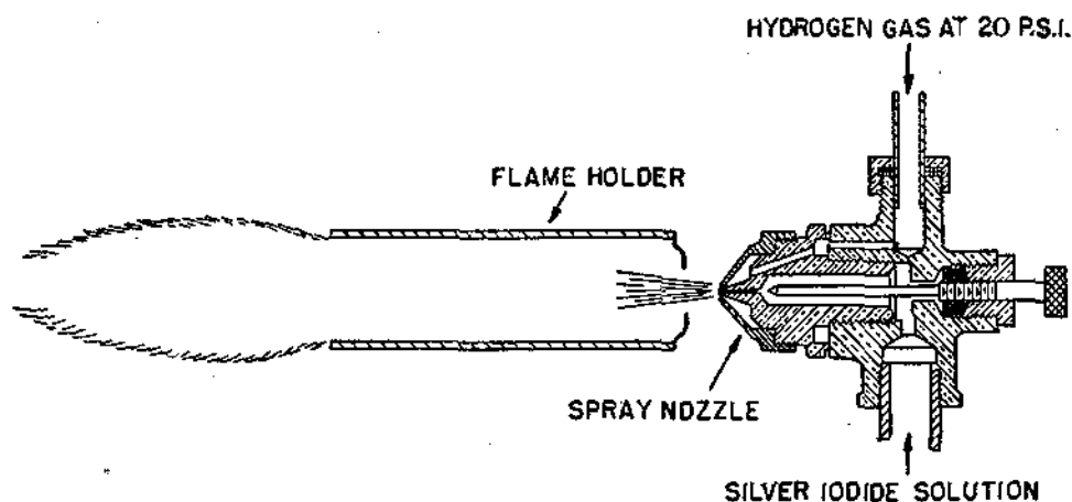
FIG. 3. Silver iodide smoke generator
