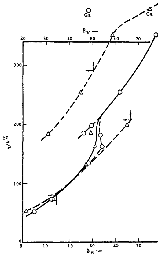
FIG. 2. Comparison of the correlation (\gamma/V^{1/3}) vs. \delta_E (O) and (\gamma/V^{1/3}) vs. \delta_V ( \Delta ) of several liquid metals.
