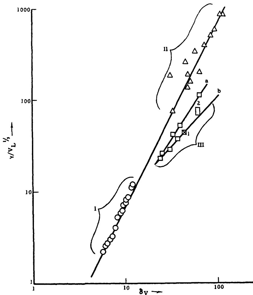
FIG. 1. Relation between surface free energy density ( \gamma/V_L^{1/3} ) and the cohesive energy density parameter \delta_V [ =(\Delta E_{vap}/V_L)^{1/2} ] for (I) spherical organic molecules and non-metallic elements, (II) metals, and (III) inorganic salts and oxides (1 = lead monoxide; 2 = silicon dioxide).
