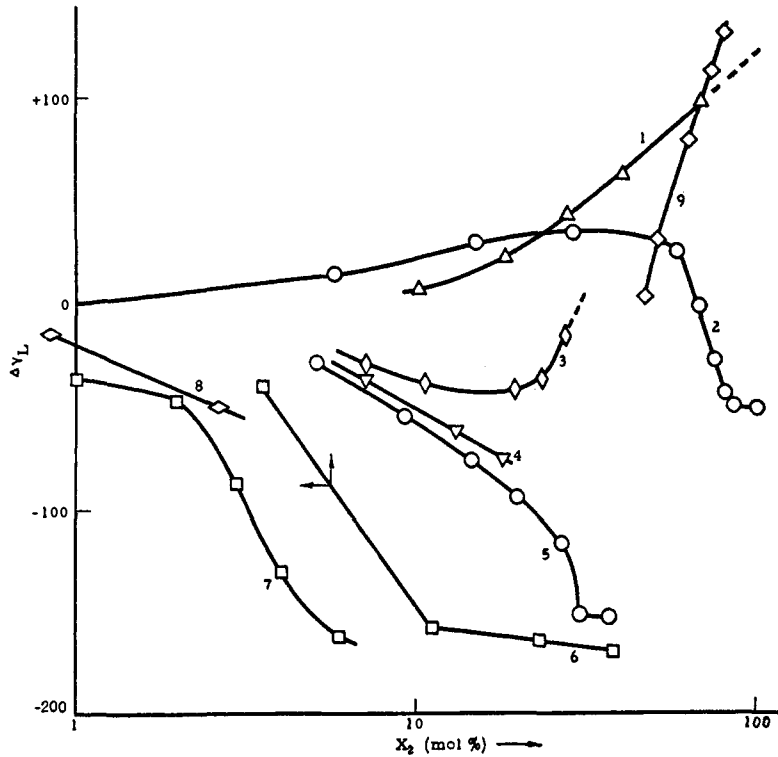
FIG. 5a. Change in surface tension ( \Delta\gamma_L ) of fused metal oxides by addition of various other metal oxides ( X_2 = mole per cent of solute).
