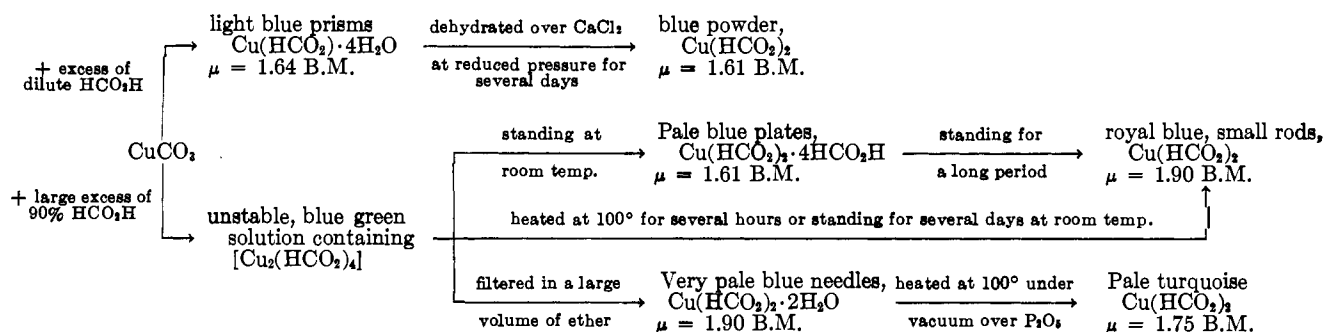
Fig. 16.—Diagram of the preparation method of the modifications of copper(II) formate.
