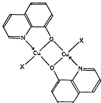
Fig. 15.—The proposed binuclear structure of copper(II) compounds with 8-hydroxyquinoline and X; X = Cl, Br, or \text{NO}_3 .
