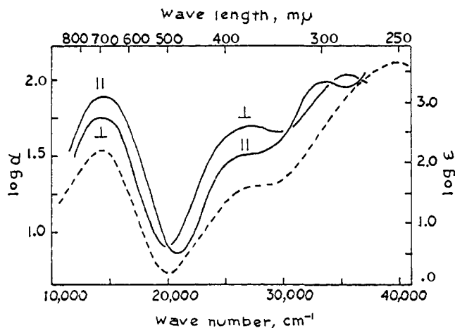
Fig. 7.—Absorption spectra of copper(II) acetate monohydrate in the crystalline state (left scale, —): || absorption with the light polarized in the complex plane, ⊥ absorption with the light polarized along copper-copper linkage. Absorption in ethanol (right scale, - - - -).
