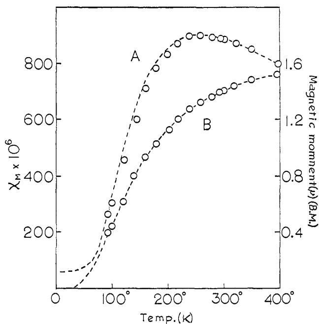
Fig. 2.—Magnetic susceptibilities ( \chi_M ) and magnetic moments ( \mu ) of copper(II) acetate monohydrate: ----, theoretical curves; curve A, magnetic susceptibilities; curve B, magnetic moments; O, experimental values.
