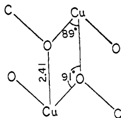
Fig. 18.—Dimeric configuration of N,N'-disalicylideneethylenediaminecopper(II).
