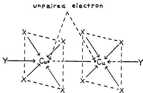
Fig. 6.—Configuration of copper(II) ions in the alkanoates.
