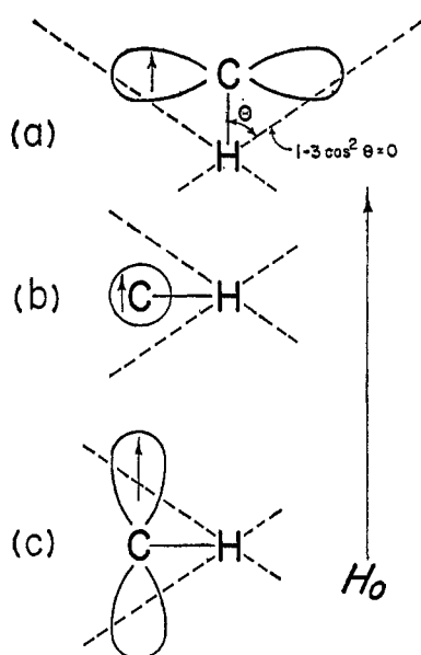
Fig. 4.—The origin of anisotropic hyperfine interaction with \alpha -protons: (a) H_0 parallel to C-H _{\alpha} bond, (b) H_0 perpendicular to C-H _{\alpha} and to p-orbital, (c) H_0 perpendicular to radical plane.
