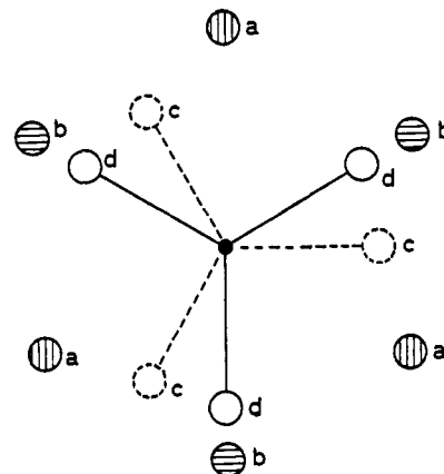
Figure 5.—Projection along the c axes of a rhombohedral cell to illustrate a possible relation, discussed in the text, between phases III and I of potassium nitrate. Small central circle, nitrogen atom; shaded circles ( a and b ), cations; open circles ( c or d ), oxygen atoms. The size of the circles has no significance. In position c , an oxygen atom is intermediate between an a and b cation. In position d , the oxygen atoms are in the same plane as one set of cations ( e.g. , a ).
