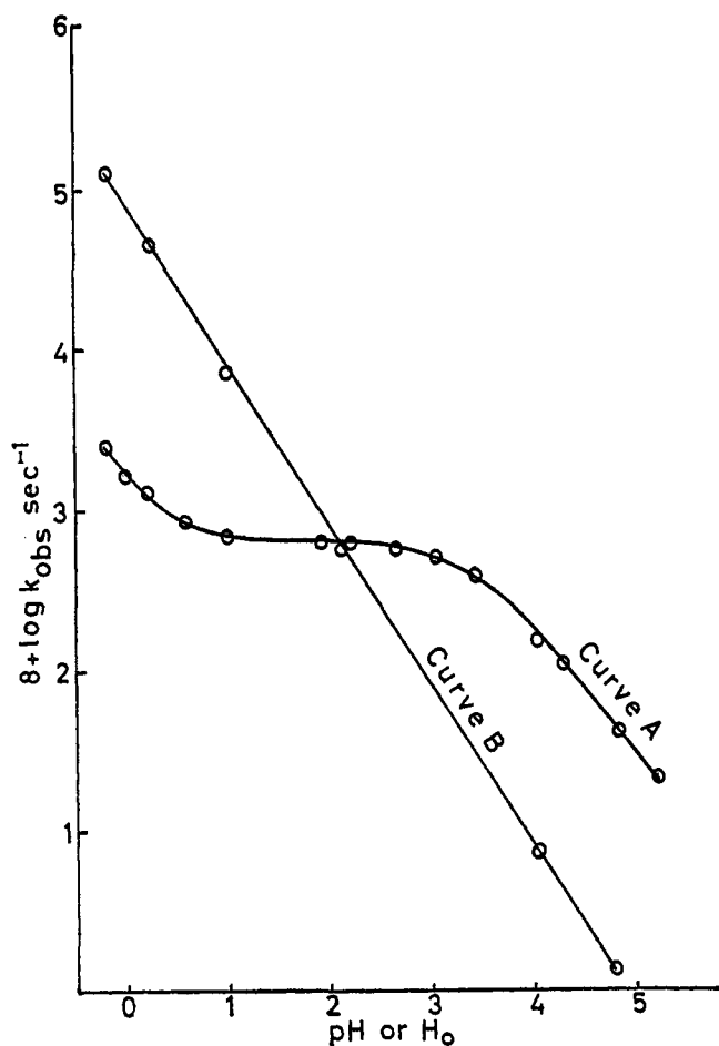
Figure 1. Plot of \log k_{\text{obs}} vs. pH or H_0 for the hydrolysis of 2-naphthyl- \beta -D-glucopyranosiduronic acid (curve A) and 2-naphthyl- \beta -D-glucoside (curve B) at 90.1°.
