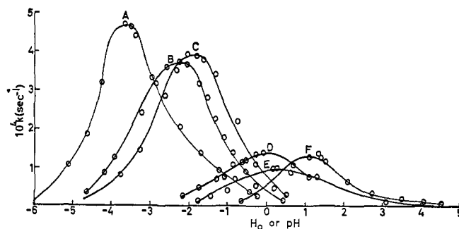
Figure 5. The dependence on pH and H_0 of the rate constant for the hydrolysis of N -aryl-D-glucosylamines at 25°C: (A) p -nitrophenyl, (B) p -carboxyphenyl, (C) p -trifluoromethylphenyl, (D) phenyl; (E) p -tolyl, (F) p -hydroxyphenyl.
