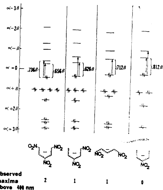
Figure 6. Orbital energy levels in nitrocyclohexadienates and nitropropenide \sigma complexes (adapted from ref 103 and 104 with permission of the author).
