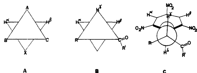
Figure 2. Representation of an asymmetric environment in an anionic \sigma complex.
