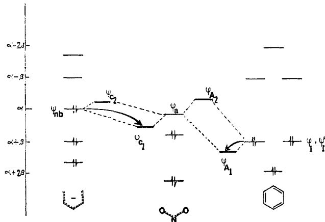
Figure 8. Orbital energies for interaction of a NO 2 group with pentadienyl anion and benzene (adapted from ref 23 with permission of the authors).
