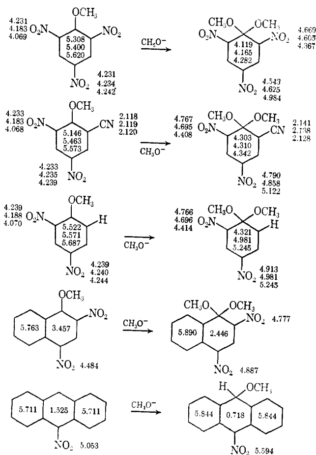
Figure 7. Electron populations for various nitro aromatics and their corresponding \sigma complexes with methoxide. Values from top to bottom represent dihedral angles of 0 , 30 , and 60^\circ (for the bicyclic and tricyclic systems; only the value for \omega = 0^\circ was calculated). This figure is adapted from ref 23 with permission of the authors.
