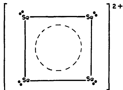
Figure 5. Structure of \text{Se}_4^{2+} in \text{Se}_4(\text{HSO}_7)_2 . 192
