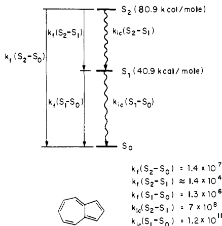
Figure 2. Spectroscopic data for azulene.
