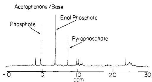
Figure 6. 40.5-MHz ^{31}\text{P} NMR spectra of products formed from the fragmentation of 25 mg of dihydrogen threo -1-phenyl-1,2-dibromopropylphosphonate (I) at room temperature in 3.0 mL of acetophenone mixed with 1.0 mL of 2,2,6,6-tetramethylpiperidine. Chemical shifts are relative to an external standard of 85% phosphoric acid; upfield shifts are assigned a negative sign.
