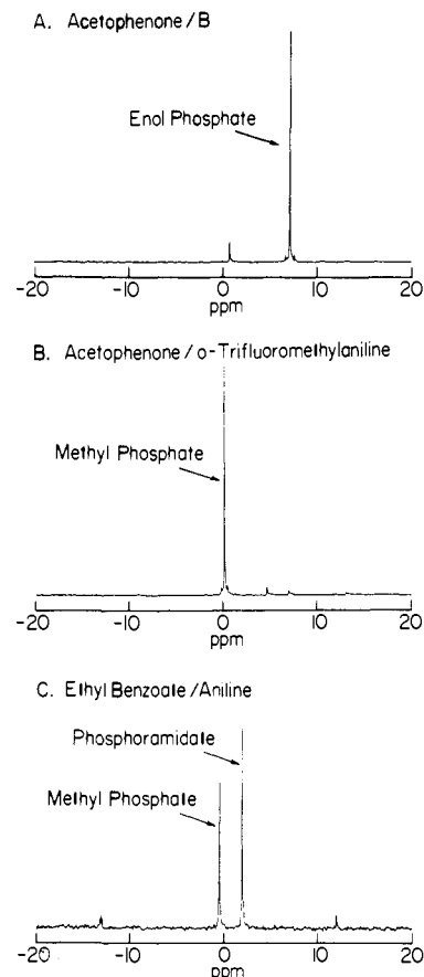
Figure 3. 40.5-MHz 31 P NMR spectra of products formed from the fragmentation of 25 mg of methyl hydrogen erythro -1-phenyl-1,2-dibromopropylphosphonic acid (I) at 70 °C in (A) 3.0 mL of acetophenone mixed with 50 μL of 2,2,6,6-tetramethylpiperidine, (B) 3.0 mL of acetophenone mixed with 0.30 mL of o -(trifluoromethyl)aniline and 50 μL of 2,2,6,6-tetramethylpiperidine, and (C) 3.0 mL of ethyl benzoate mixed with 0.30 mL of aniline and 50 μL of 2,2,6,6-tetramethylpiperidine. Chemical shifts are relative to an external standard of 85% phosphoric acid; upfield shifts are assigned a negative sign.
