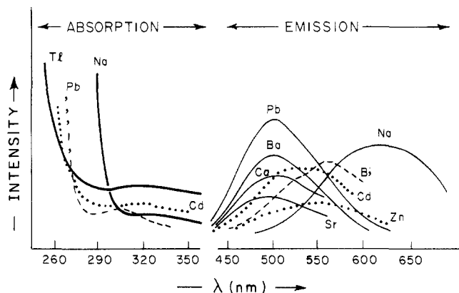
Figure 11. Absorption (300 K, aqueous solution) and emission (77 K, single crystal) of various molybdate salts. The higher energy absorption edges are onsets of intense singlet ← singlet absorption intensity of the anion, \lambda_{\max} 227 nm. The variation of absorption edge is largely attributable to the different concentrations required to observe the weak side bands in the 250–350-nm region. The behavior of the tungstates is very similar except that maxima occur 30–50 nm to higher energy.
