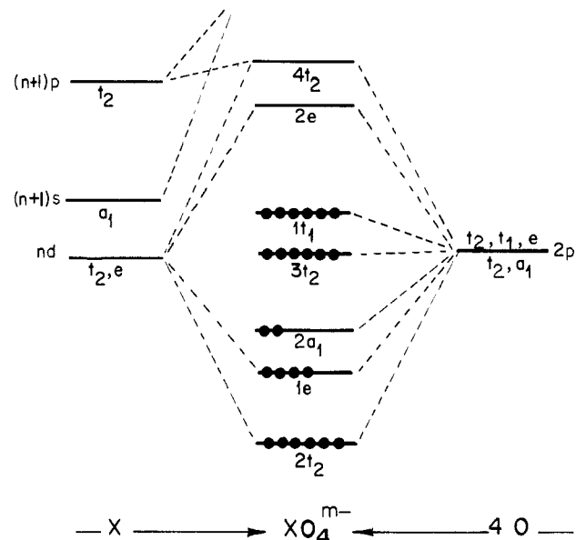
Figure 9. A schematic MO energy level diagram for a 32-electron T_d ion or molecule, XO_4^{m-} . n denotes the principal quantum number. The 3t_2 MO usually contains little or no 4d character, and for that reason no compositional connection to nd is shown. A similar comment applies to the (n+1)s/2a_1 compositional connection.
