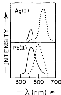
Figure 8. Emission spectra of two thiocyanates in aqueous glass (solid line) and in crystal (dotted line) at 77 K. The crystal systems have \tau_p \approx 5 \times 10^{-3} s, whereas the aqueous systems have \tau_p \approx 5 \times 10^{-1} s.
