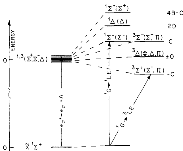
Figure 6. The {}^1\text{LE} and {}^3\text{LE} states of \text{NCO}^- and their MO genesis. The parameters \epsilon_{\pi^*} , \epsilon_{\pi} , A , B , C , and D are defined in Wittel et al. 36 The scheme shown here is based on A \gg B = C = D . The state symbolics in the upper right are {}^{2S+1}\Gamma in C_{\infty v} ( \Gamma in C_{\infty v}^* , where C_{\infty v}^* is the double group). This same diagram applies to \text{NCS}^- and \text{N}_3^- , with appropriate changes to D_{\infty h} and D_{\infty h}^* in the latter case.
