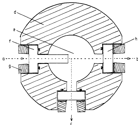
Figure 2. Scheme of a fluorescence cell (after Lakowicz and Weber 26 ). a = excitation beam, b = transmission beam, c = emission beam, d = steel cell housing, e = sample compartment, f = T-shaped quartz window, g = holding screw, h = cylindrical quartz window.
