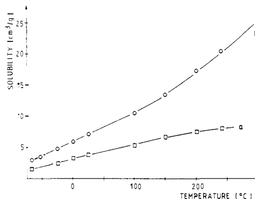
Figure 14. Solubility of hydrogen in toluene: 37a (a) 50-bar H_2 pressure; (b) 100-bar H_2 pressure.
