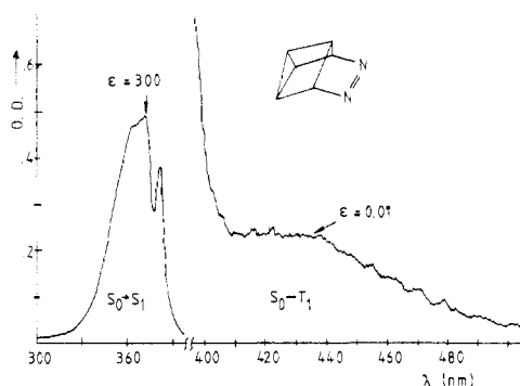
Figure 10. UV absorption spectrum of azo compound 1 in pentane. 51 S_0 \rightarrow S_1 spectrum with 1-cm pathlength; S_0 \rightarrow T_1 spectrum with 10-cm pathlength. The spectra are similar in the presence or absence of oxygen.
