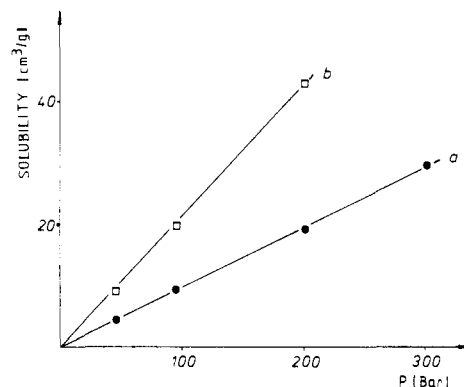
Figure 13. Solubility of hydrogen in cyclohexane: 37a (a) at 25 °C; (b) at 150 °C.
