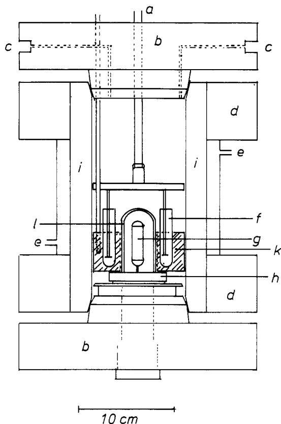
Figure 7. Multiple sample UV autoclave. 66b a = magnetic stirrer, b = autoclave lid, c = gas exit and entrance, d = flange, e = connection to thermostat, f = sample test tube, g = lamp, h = quartz tube holder, i = autoclave housing, k = sample holder, l = pressure-stable quartz tube.
