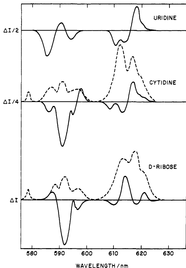
Figure 4. CPL spectra (solid line traces) and unpolarized emission spectra (broken line traces) obtained in the {}^5D_0 \rightarrow {}^7F_0 , {}^7F_1 , and {}^7F_2 transition regions of \text{Eu}^{3+} . Spectra were obtained on aqueous solutions at pH \sim 6.8 with 1:3 [\text{Eu}^{3+}]:[\text{ligand}] ratios and [\text{Eu}^{3+}] = 10 \text{ mM} .
