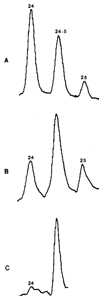
Figure 8. Charge stripping region of Hg/O 2 (30% T) NR spectra of (A) CH_3^{35}Cl^+ , (B) CH_2^{35}ClH^+ , and (C) CH_2^{35}Cl^+ . Peak heights of m/z 24.5 relative to those of the reionized precursor are (A) 0.025%, (B) 0.11%, and (C) 0.29%. The ^{35}Cl isotopomers are used for increased sensitivity. The NR spectra of the ^{35}Cl and ^{37}Cl isotopomers are identical within experimental error.
