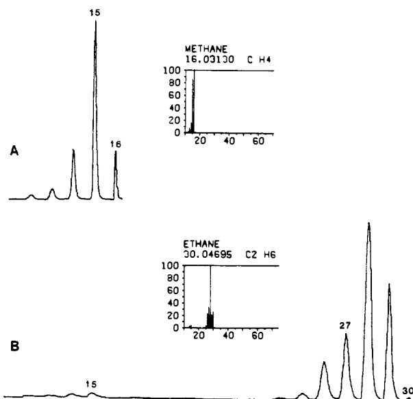
Figure 14. Hg/O 2 NR spectra of (A) \text{CH}_4^{\cdot+} and (B) \text{C}_2\text{H}_6^{\cdot+} . Inset: EI spectra.
