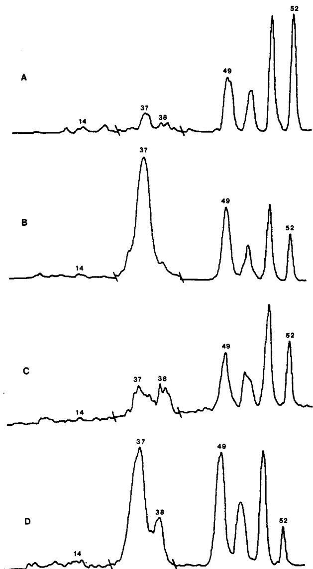
Figure 6. Hg/He NR spectra of \text{H}_3\text{C}^{37}\text{Cl}^{++} (A, B) and \text{H}_2\text{C}^{37}\text{ClH}^{++} (C, D) at transmittances with He of 90% (A, C) and 30% (B, D).
