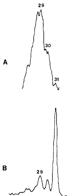
Figure 7. Partial MI/O 2 (50% T) NR spectra of (A) (CH 3 O) 2 CHN(CH 3 ) 2 •+ and (B) HOCH 2 CH 2 N(CH 3 ) 2 •+ .
