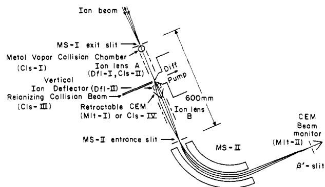
Figure 1. Neutralization-reionization interface: (Cl) collision region; (Dfl) ion deflector; (MIt) channel electron multiplier.
