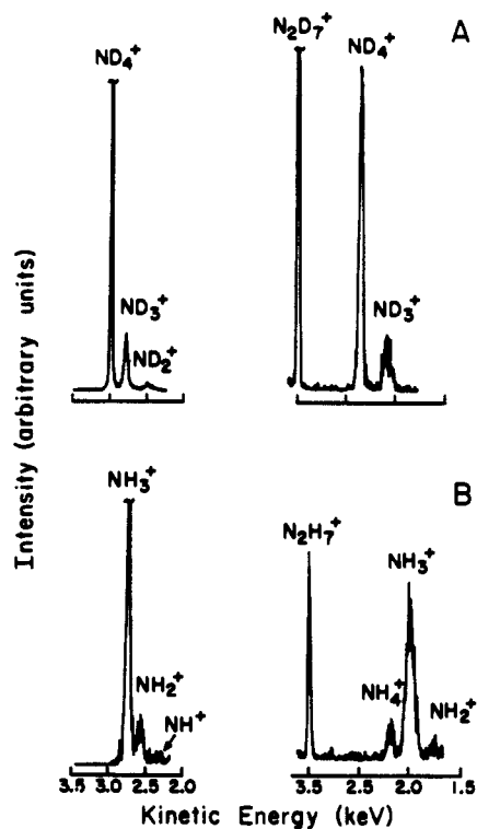
Figure 10. Na/NO 2 NR spectra of (A) ND 4 + and ND 4 (ND 3 ) + and (B) NH 4 + and NH 4 (NH 3 ) + .
