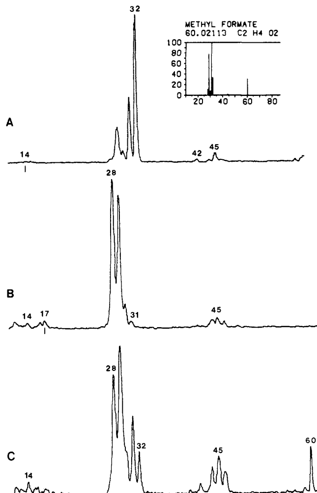
Figure 2. (A) CAD/He spectrum of \text{HCO}_2\text{CH}_3^{+\bullet} . (Inset) EI spectrum of methyl formate. (B) He/ \text{O}_2 and (C) Hg/ \text{O}_2 NR spectra of \text{HCO}_2\text{CH}_3^{+\bullet} .
